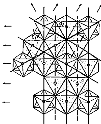
Fig. 1. Sheet of [M_3\phi_2(TO_4)_2] showing some of the symmetry elements in space group P\bar{3}m1 and the unit cell outline with a_1, a_2 \sim 6 \text{ \AA} . Some symmetry elements m, \bar{1}, 2, 3 and axial glides are shown and are slightly offset to ease visualization of the sheet.
