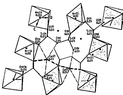
Fig. 5e. Representation of the macfallite structure down [010].
