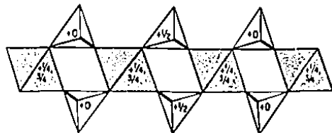
Fig. 2b. Alternative projection of 2[M_2O_4(TO_4)_2] , a frequent projection for the Fig. 5 series. The edge-sharing LM\phi O_T , 6\text{\AA} octahedral chains are normal to the paper. The 9\text{\AA} direction runs from left to right and the intersheet portion runs from north to south. Heights are given as fractional coordinates of the 6\text{\AA} direction.
